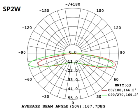
Wave pattern of the optical Lens for the modules
